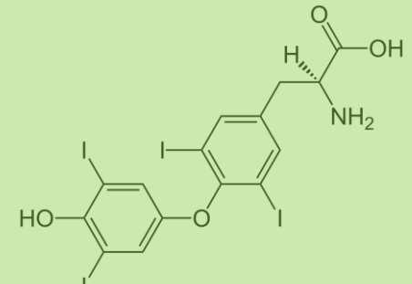
thyroxine
